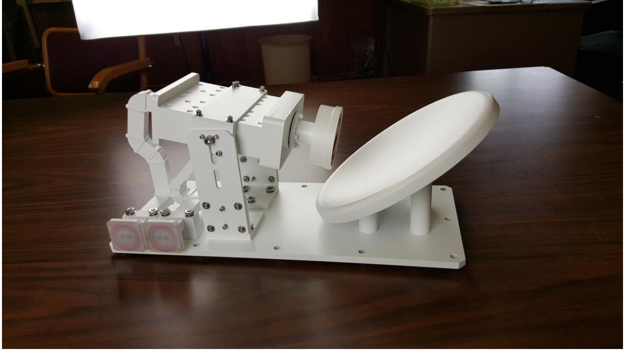
8-12 GHz, Dual Linear, Offset
